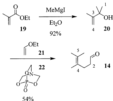
Scheme 3. Synthesis of 4,5-dimethylhex-4-enal ( 14 ) by Saucy–Marbet reaction
