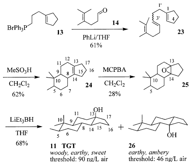
Scheme 4. Wittig–Schlosser olefination of 14 , acid-catalyzed cyclization of the resulting triene 23 , epoxidation, and subsequent reduction of 25 to the target structure 11
