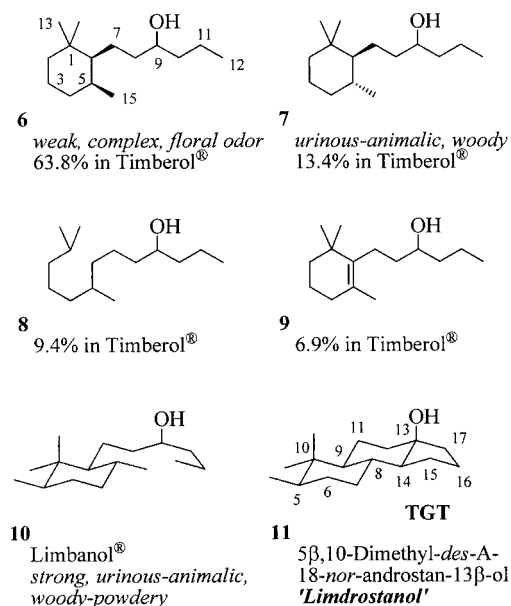
Figure 2. Timberol® components 6–9 , Limbanol® ( 10 ), and the des-A -18- nor -androstanol target molecule 11 , our so-called Limdrostanol, which was proposed to be the scaffold of 7 and 10
