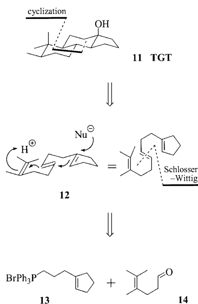
Scheme 1. Retrosynthetic analysis of the target compound 11
