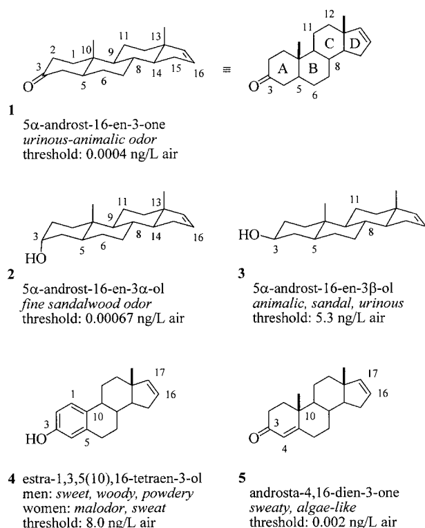
Figure 1. Steroids 1–5 with putative pheromone function in humans
