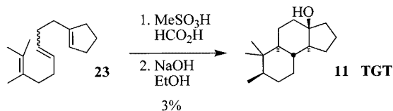
Scheme 5. Direct synthesis of the target compound 11 from the triene 23
