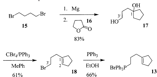
Scheme 2. Synthesis of the 3'-cyclopent-1-enylpropyl Wittig salt 13 from 1,4-dibromomethane ( 15 ) and \gamma -butyrolactone ( 16 )
